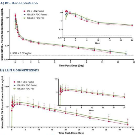
Figure 2. Arithmetic Mean (SD) Plasma Concentration-Time Profiles of (A) ISL and (B) LEN After a Single Dose of ISL and LEN Single-Agent Co-Administration Under Fasted Conditions, and ISL/LEN FDC Under Fasted or Fed Conditions a
